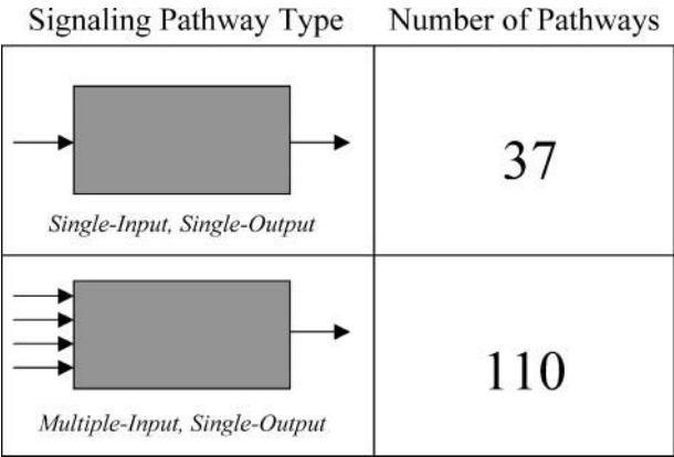
FIGURE 2 Signaling pathway types in the JAK-STAT network. Other signaling types, not present in this network, include signal pleiotropy (one-input, multiple-outputs) and cross talk (multiple inputs, multiple outputs).
